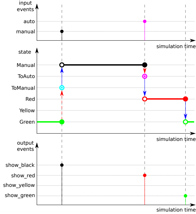
Figure 10: Trace of the autonomous traffic light.
