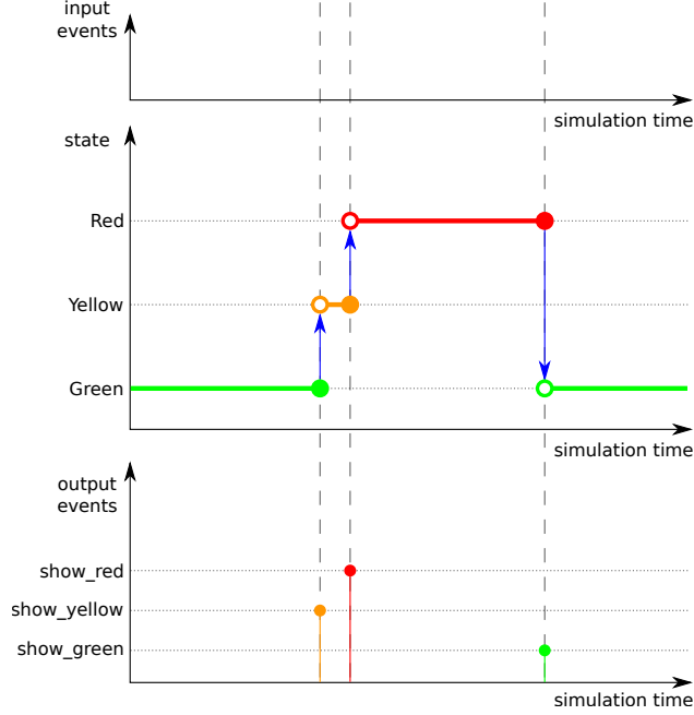
Figure 6: Trace of the autonomous traffic light with output.
