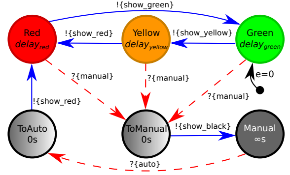
Figure 11: Model generating the trace in Figure 10.
