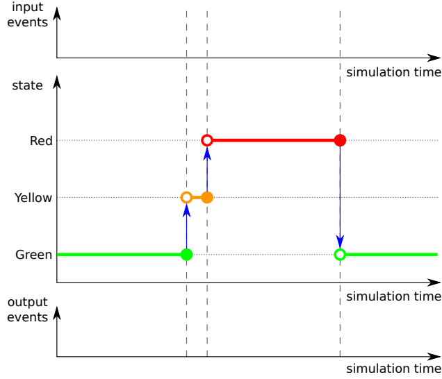
Figure 2: Trace of the autonomous traffic light.
